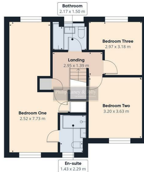
Floor 1 Building 1
