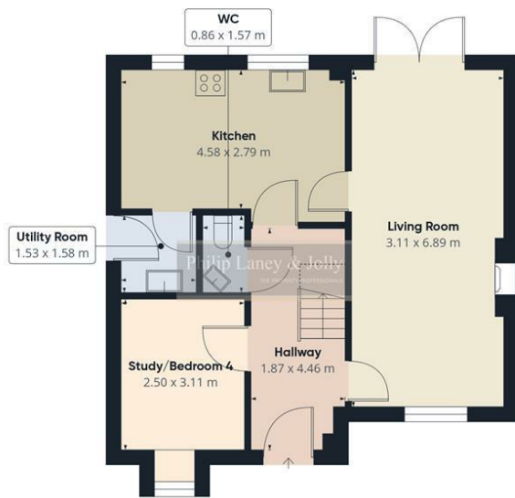
Floor 0 Building 1
